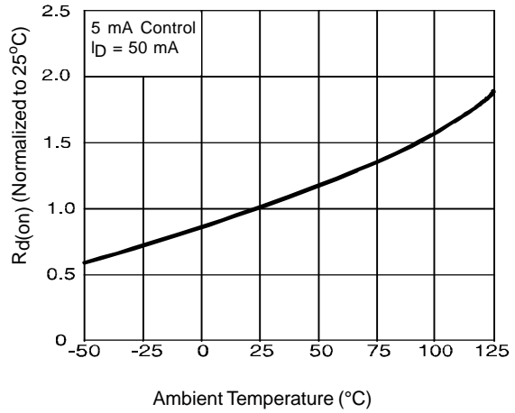
Figure 2. Typical Normalized On-Resistance
